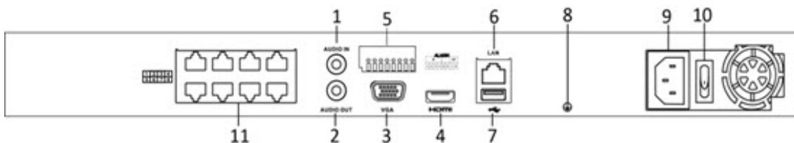
ST-EZ8 Shown above, ST-EZ16 has 16 PoE Ports
