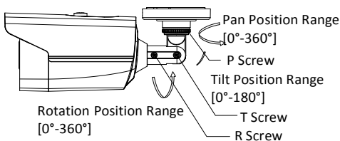
Figure 2-7 3-axis Adjustment
