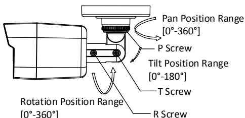
Figure 2-2 3-axis Adjustment
