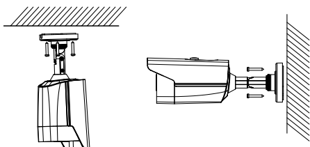
Figure 2-6 Fix the Camera to the Ceiling/Wall
