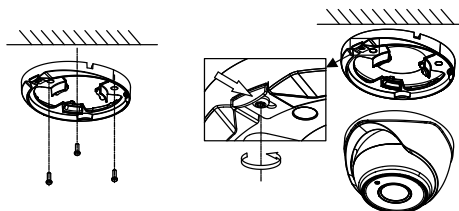
Figure 2-9 Install the Turret Camera
