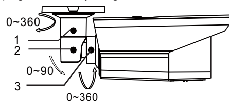
Figure 2-8 3-axis Adjustment
