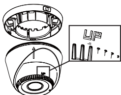
Figure 2-3 Secure the Camera
