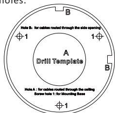
Figure 2-6 Drill Template
