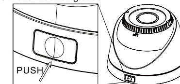
Figure 2-2 Release The Lock Screw
