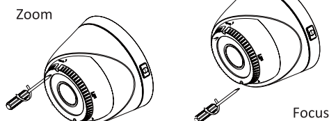
Figure 2-5 Zoom and Focus Adjustment
