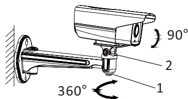
Figure 2-8 Angle Adjustment
