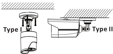
Figure 2-2 Fix the Camera to the Ceiling
