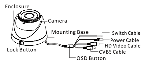
Figure 1-1 Overview of Type I Camera
