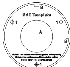
Figure 2-5 Drill Template
