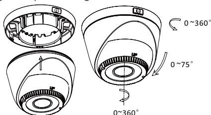
Figure 2-3 3-axis Adjustment
