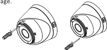
Figure 2-4 Zoom and Focus Adjustment
