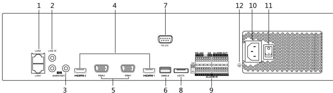
Figure 1. 3 Rear Panel
