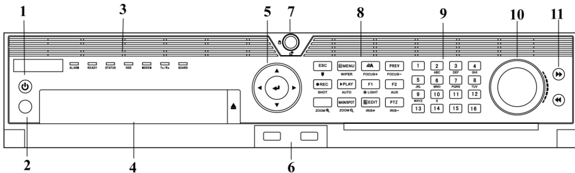
Figure 1. 1 Front Panel
