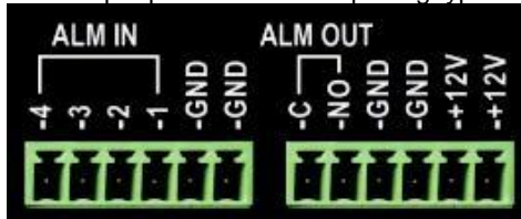
(1) Alarm input (2) Grounding (3) Alarm output (4) +12Voltage
