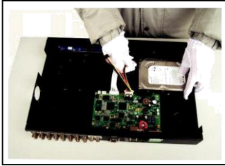
⑤connect the data wire
