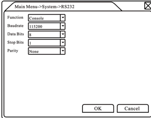
Picture 4.30 RS232 setup
