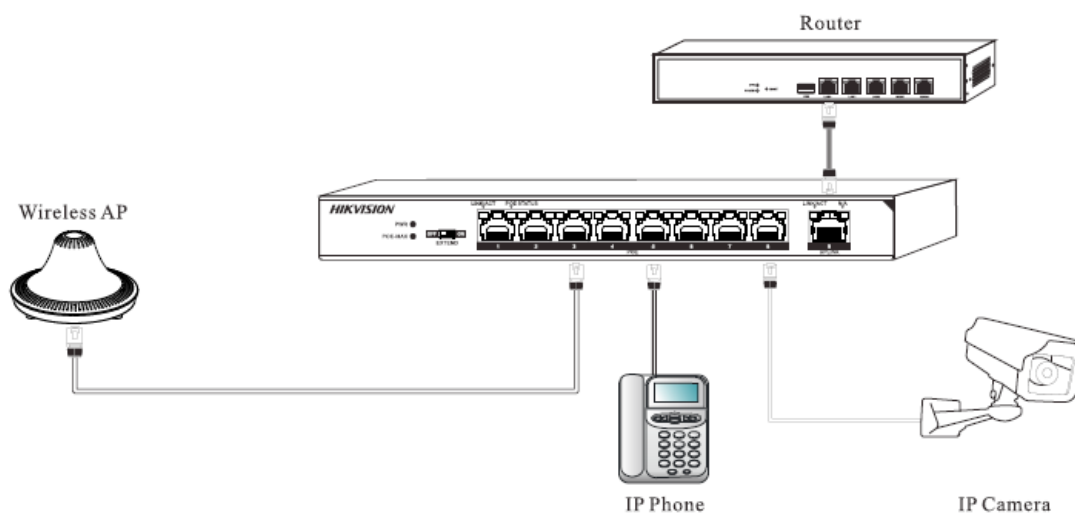
Figure 3.1 RJ45 port connection
